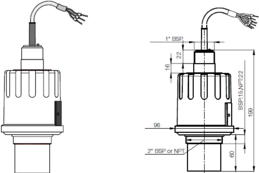
NUS-7 level transmitter for liquids – 2-wire series
